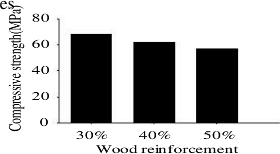
Fig.3 Compressive curves of waste wood powder and dry leaves reinforced MDI composites
