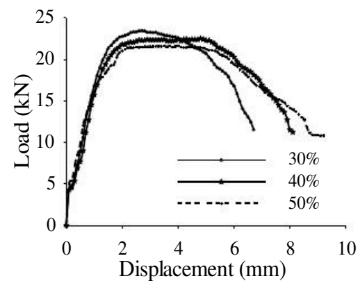
Fig.3 Compressive curves of waste wood powder and dry leaves reinforced MDI composites
